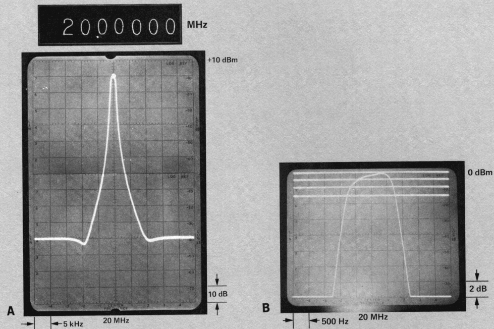
Figure 19. Filter Response.
