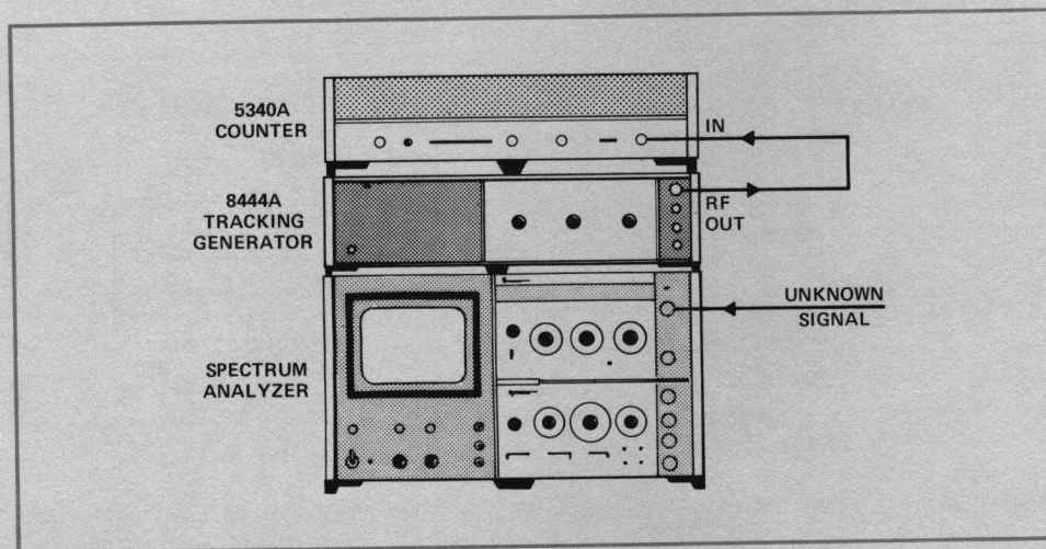
Figure 26. Frequency Counting with the 8444A.
