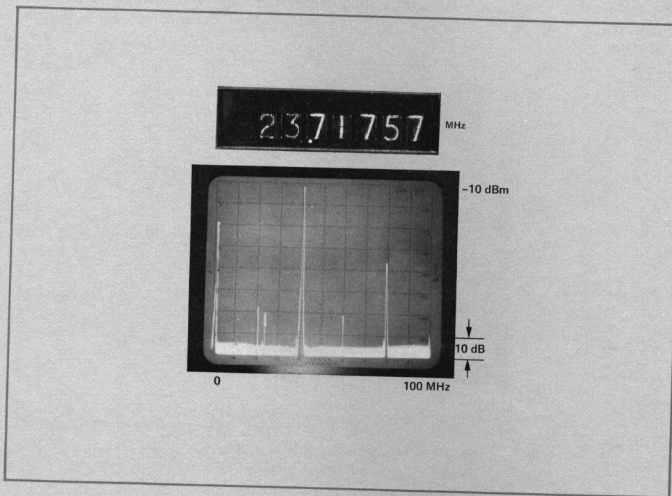
Figure 16. "Track Analyzer" Function: This CRT display shows several signals. The smallest signal ( -70 dBm) was counted by placing the marker at its peak.
