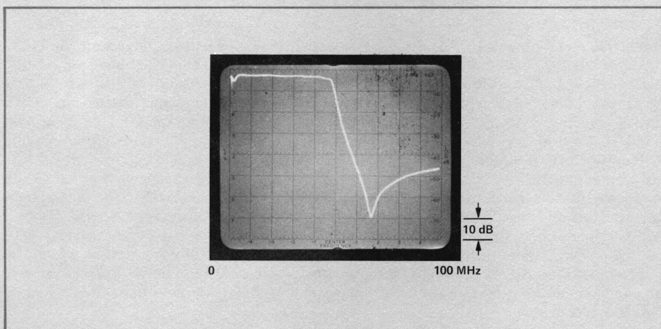
Figure 4. Low Pass Filter Response.
