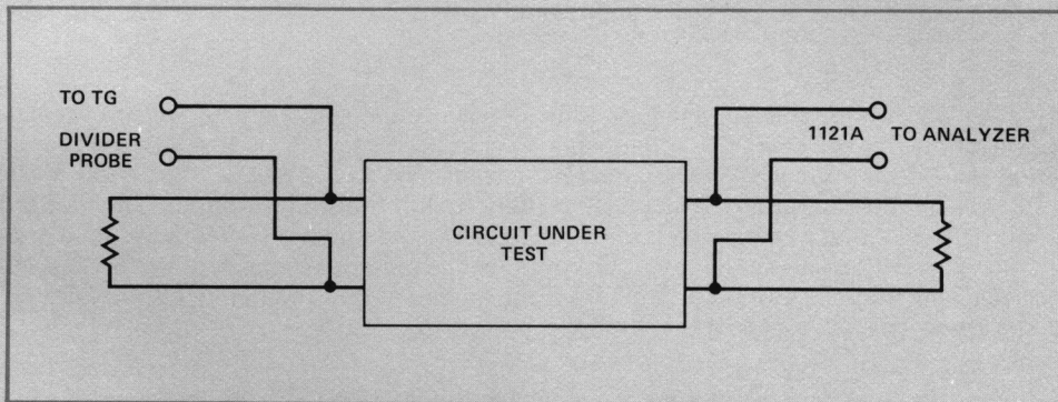
Figure 49. Probing with the Spectrum Analyzer.
