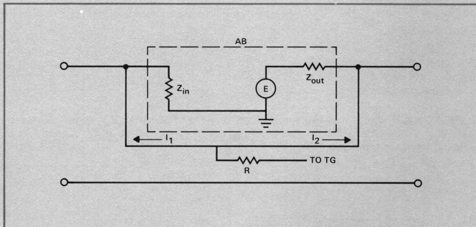
Figure 45. Current Source Simulation When Z_{out} \gg Z_{in} .
