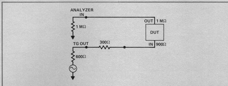
Figure 39. 900 \Omega /1 M \Omega Input/Output Device.
