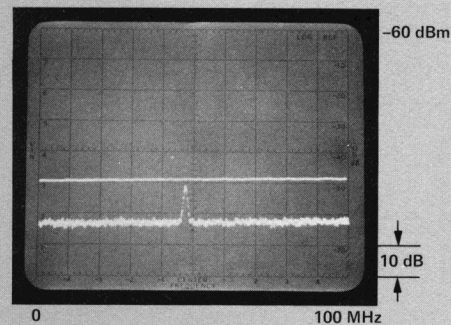
Figure 7. This signal is -111 dB. It was detected with a 1 kHz bandwidth. Notice that it could not be detected with a 30 kHz bandwidth.
