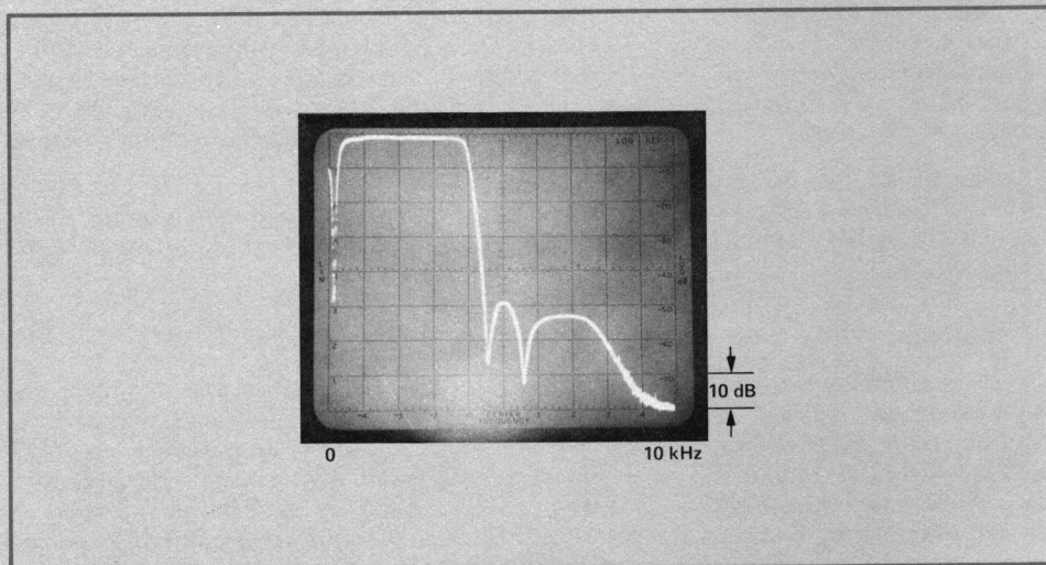
Figure 41. This CRT photograph shows the overall response of a high performance receiver. Notice how response drops sharply beyond 4 kHz.
