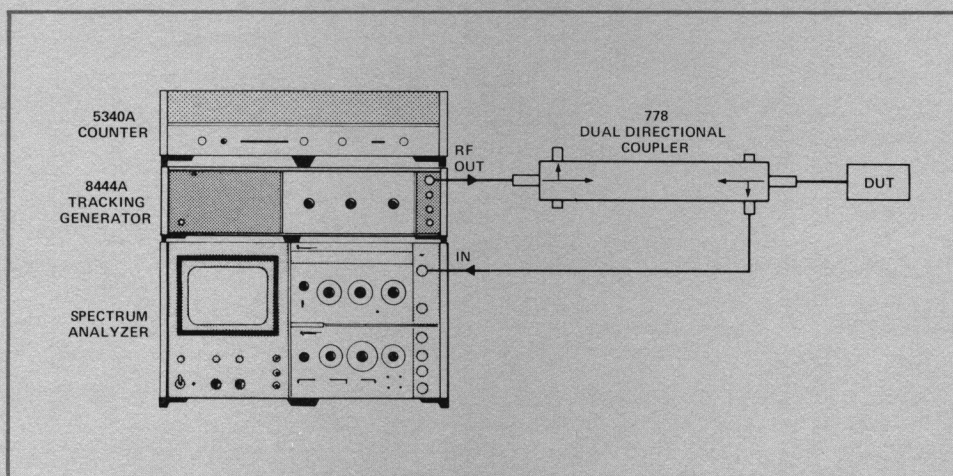
Figure 30. Return Loss Measurement with the 8444A.
